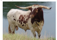
CRYSTAL IMAGE
